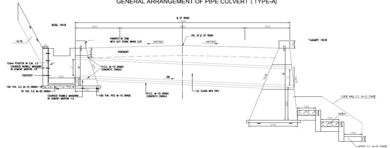
GENERAL ARRANGEMENT OF PIPE CULVERT ( TYPE-A)
