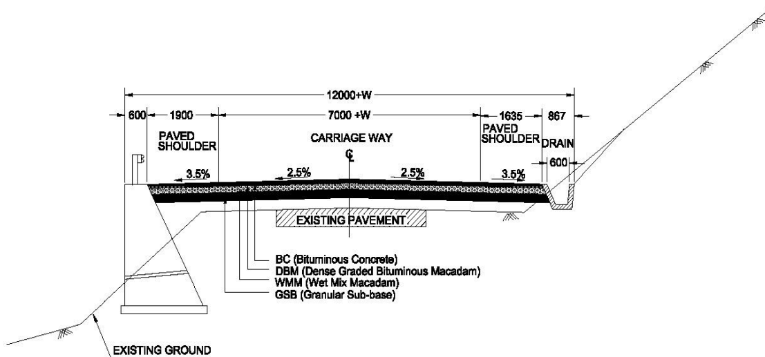
Figure 2.11(1): Typical Cross Section for Widening Primarily to Hill Side
