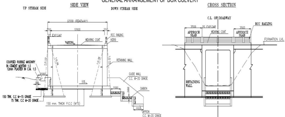
GENERAL ARRANGEMENT OF BOX CULVERT
