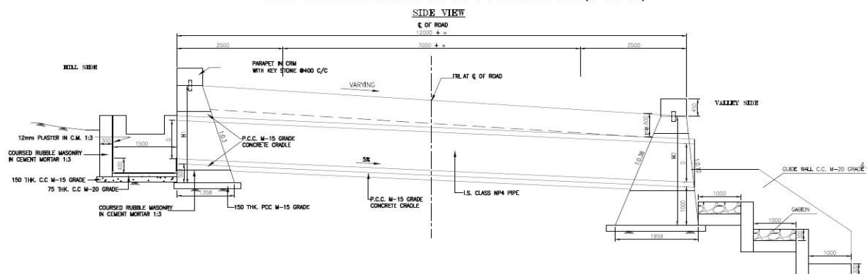
GENERAL ARRANGEMENT OF PIPE CULVERT ( TYPE-B)
